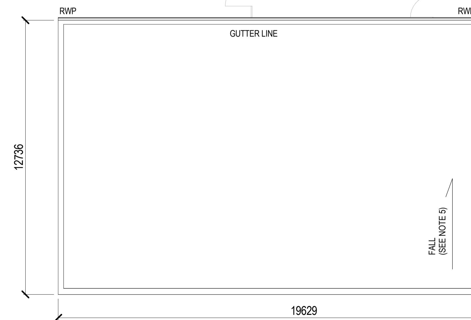
ROOF PLAN
