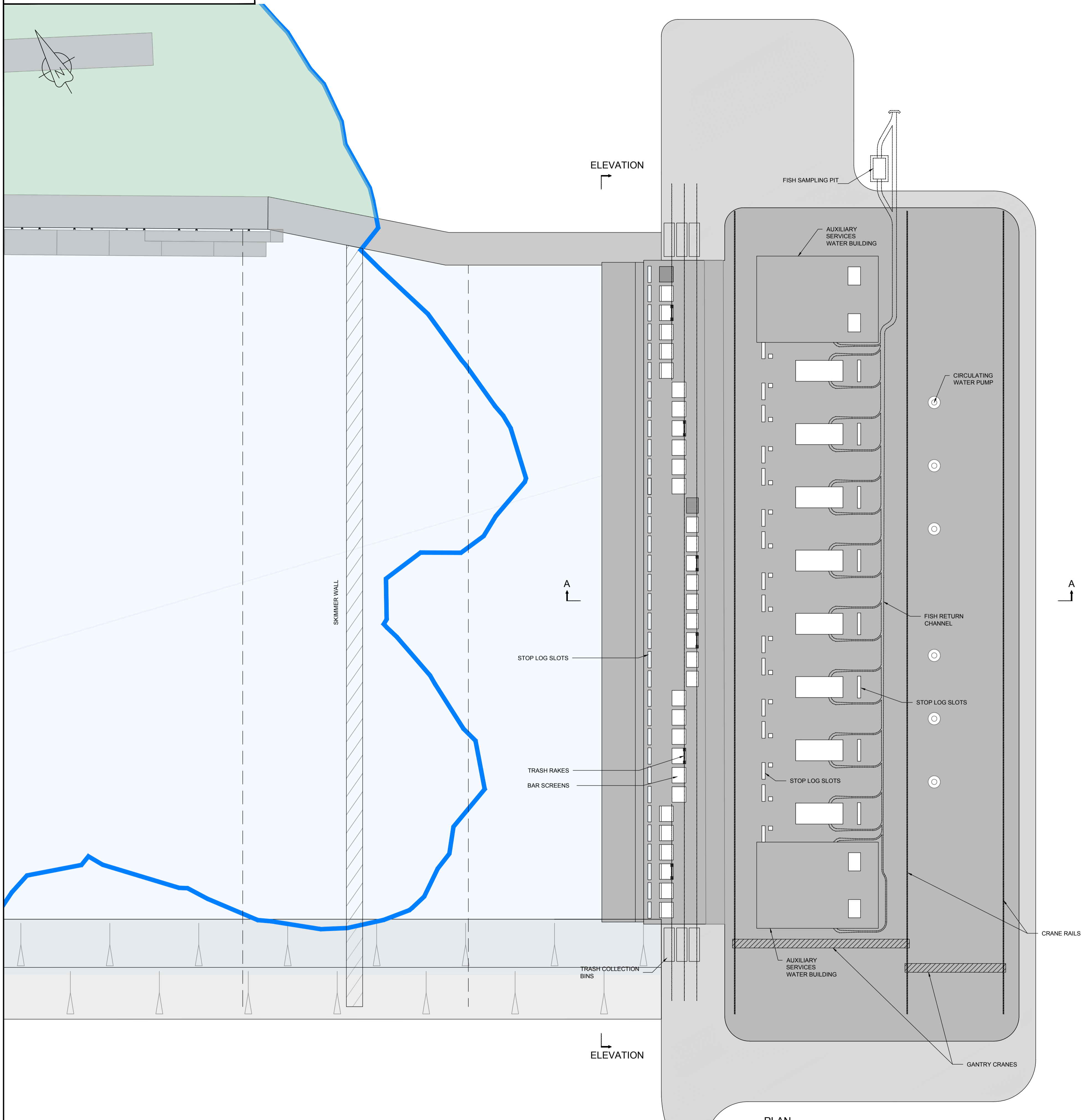
PLAN SCALE 1:500
