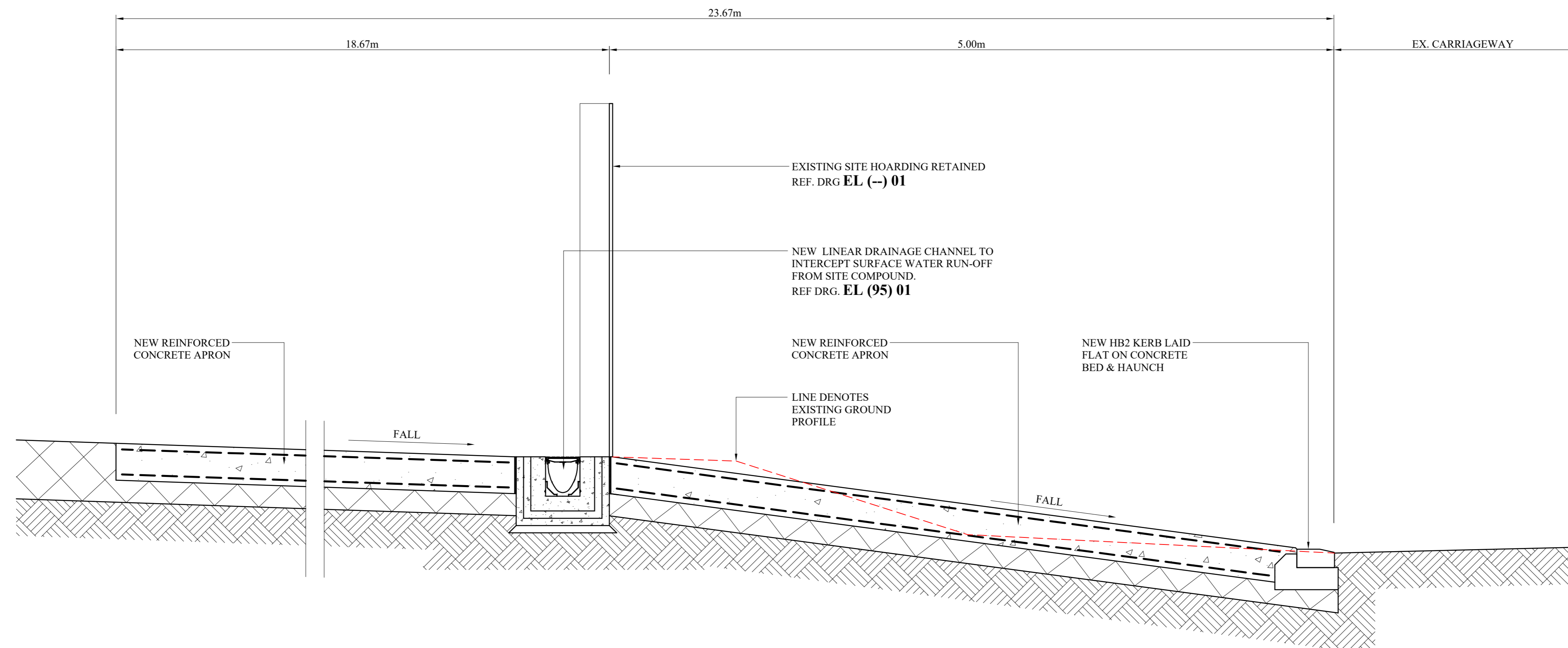
SECTION 01 TYP. SECTION THROUGH NEW CONCRETE APRON 1 : 20
